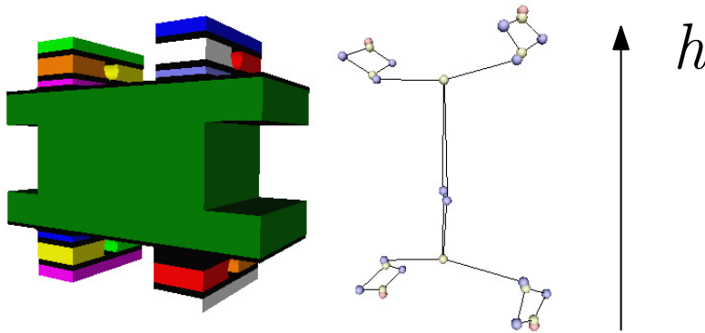
Figure 3.5: Cell decomposition approach for Extended Reeb graph construction.
