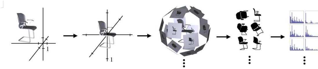
Figure 2.9: Computing the LightField descriptor of a 3D model [27].
