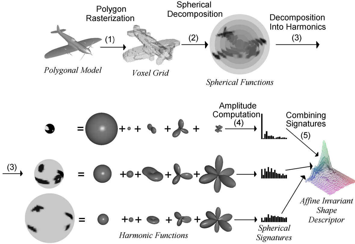
Figure 2.8: Computing the harmonic shape representation [52].
