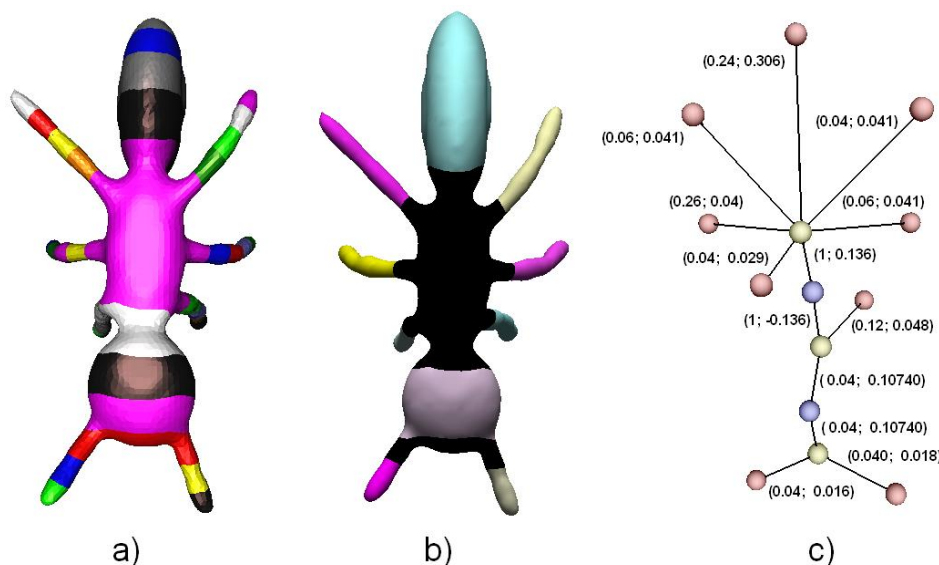
Figure 4.7: ERG construction. (a) Shape segmentation. (b) Merging simple adjacent components. (c) ERG with edge attributes: shape index and segment weight.
