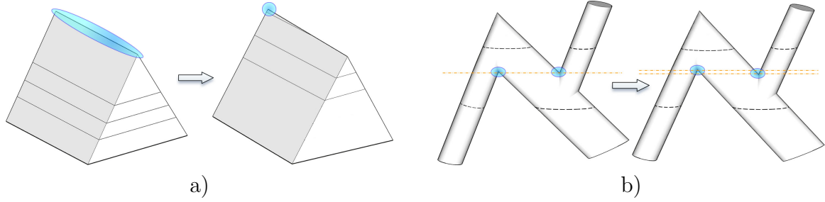
Figure 3.2: Degenerate critical points and non-degenerate critical points of a complicated Morse function. a) handling degenerate critical points by slight rotation; b) separating non-degenerate critical points with the same value of the mapping function by minor local shear.
