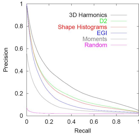
Figure 2.17: Precision Recall plot [52]. The top most plot corresponds to the most efficient retrieval.
