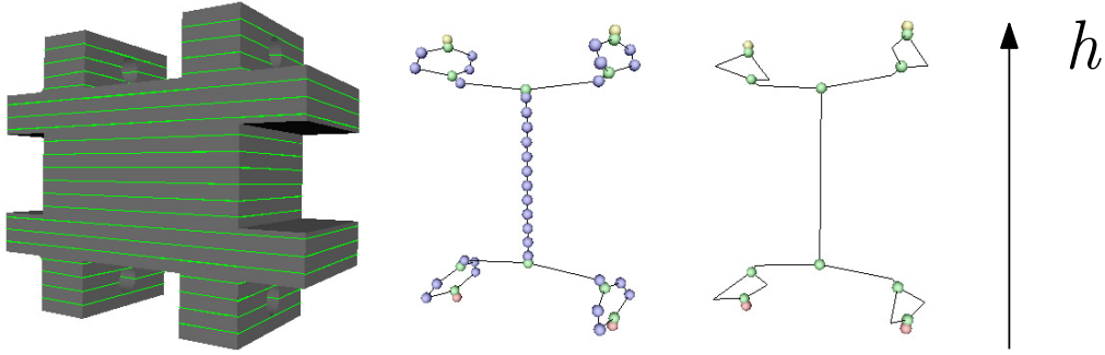
Figure 3.4: Contour driven approach for Reeb graph construction.
