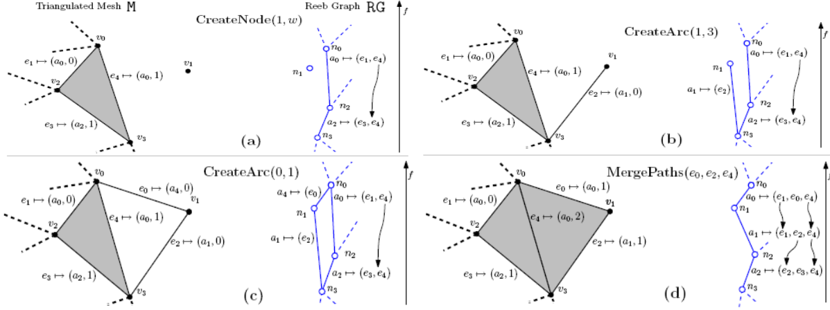
Figure 3.8: The main steps of the proposed in [71] approach for construction of the Reeb graph. a) For a new vertex v_1 insert a new node n_1 in the Reeb graph. b-c) For each new edge e_2 and e_0 insert a corresponding arc in the graph. d) For each triangle (after all its vertices and edges have been read) merge two paths a_1, a_4 and a_2, a_0 connecting the lowest and the highest vertices in the triangle.
