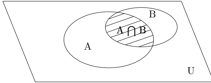
Figure 2.14: The set of all shapes U in a repository, A is the subset of all shapes relevant to a query, B is the subset of all retrieved shapes. The intersection A \cap B is the subset of shapes relevant to the query and retrieved.
