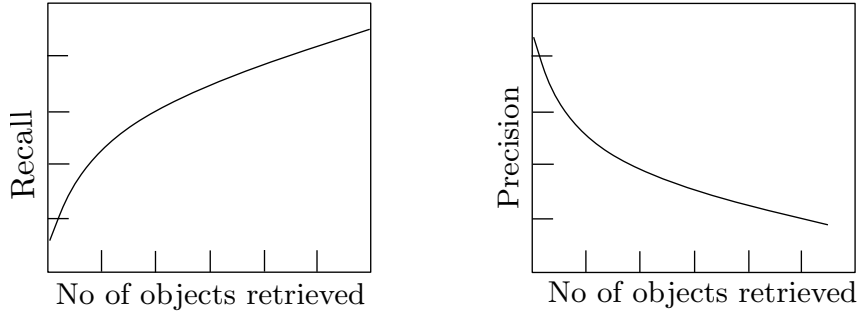
Figure 2.16: Recall and precision plots vs. the number of retrieved objects.
