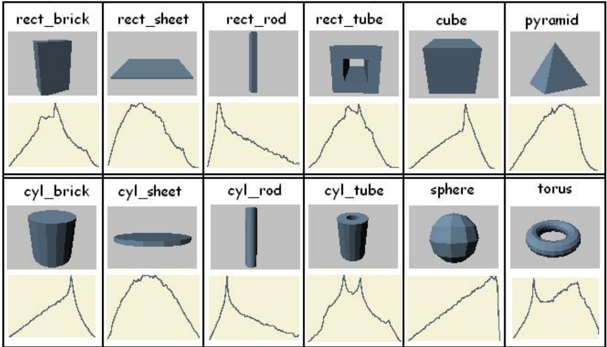
Figure 4.10: Geometrical primitives for Constructive Solid Geometry and their shape distributions.
