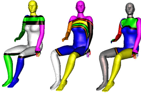
Figure 5.3: A model of a human is segmented using height, distance from the barycenter and geodesic distance measuring functions.
