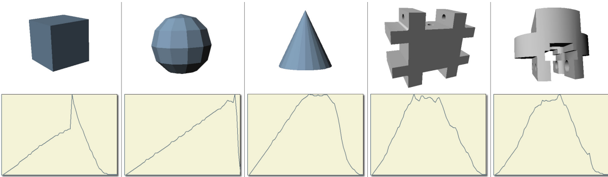
Figure 2.7: Distributions of D2 function for some 3D models. The more details are present in the shape of a model the less discriminative the distribution.
