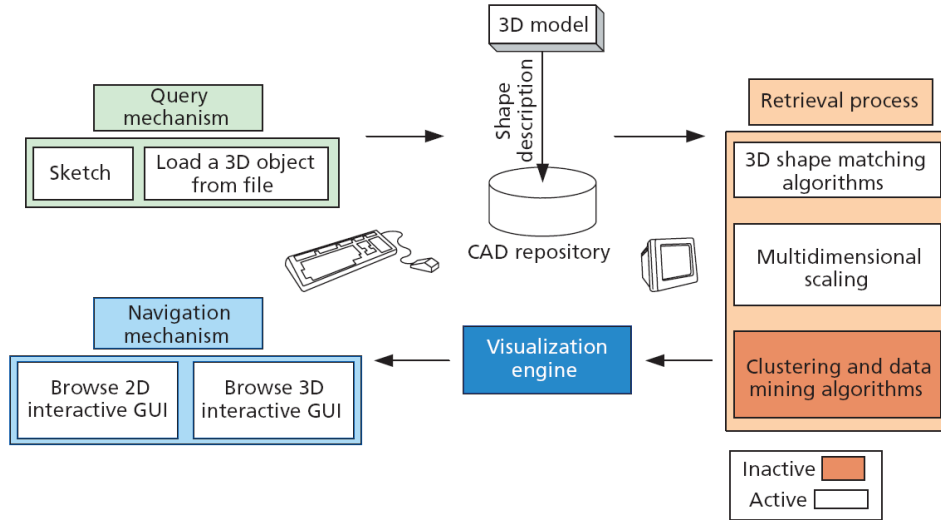
Figure 2.3: Organization of Purdue Navigation and Discovery Engine [74].
