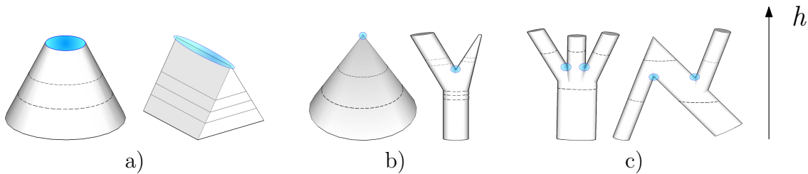
Figure 3.1: Critical points of the height measuring function. (a) degenerate critical points, (b) non-degenerate critical points with a single critical point per each critical value, (c) and with several critical points for the same critical value.
