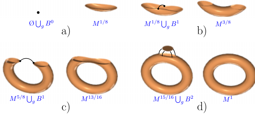
Figure 3.3: Cell decomposition of the torus. a) Attaching 0-cell corresponds to introduction of a circle. b) Attaching 1-cell corresponds to the union of two circles. c) Attaching of 1-cell corresponds to the disconnection of a circle and to formation of two new circles from one. d) Attaching 2-cell corresponds to extinguishing of a circle [45].
