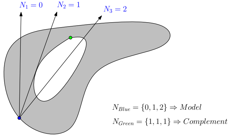
Figure 4.1: The triple parity count for the blue vertex of the contour results in 1,2 and 0 intersections. The voting result is that the contour represents the model (the majority of the intersection numbers is even). For the green vertex of the second contour the parity count gives 1 intersection for all three rays. Thus the second contour describes the complement.
